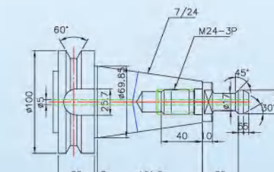
TOOL SHANK: BT50 RETENSION STUD: MAS 1
