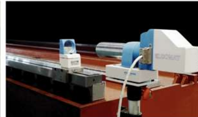
STRAIGHTNESS MEASUREMENT
